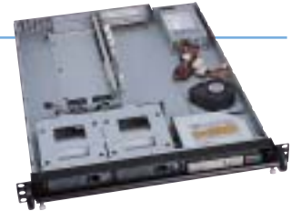
EC-1015 Support PICMG Full-size CPU Card and two PCI add-on cards
